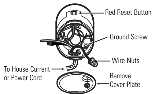
Bottom of the Disposer (end bell)
