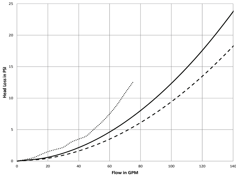
Head Loss with Valve
