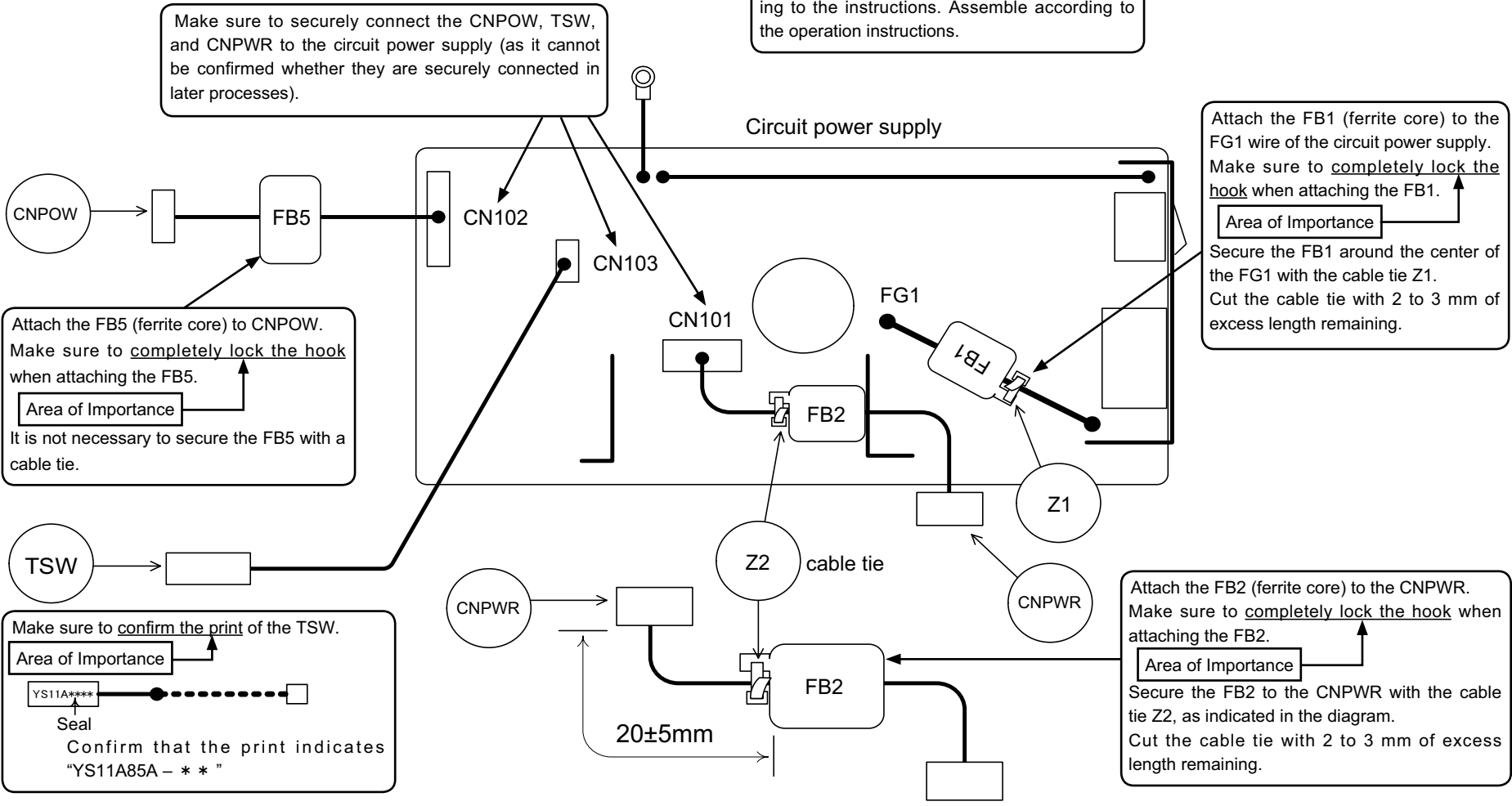
Wiring diagram 1
