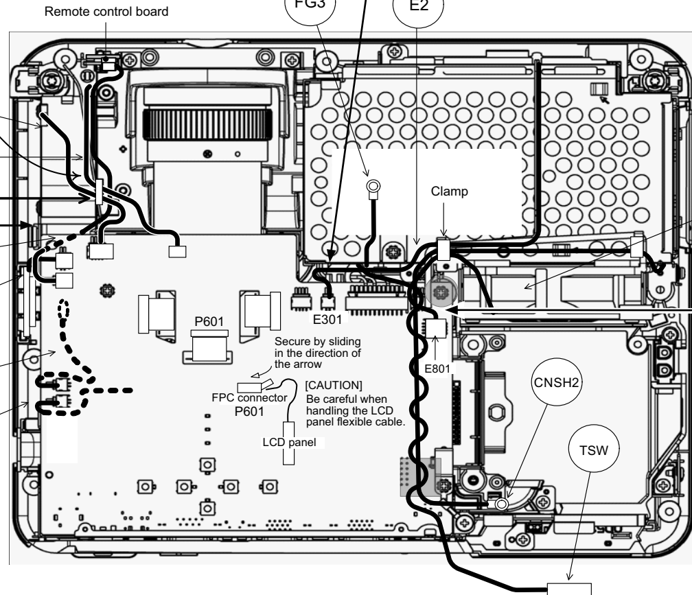
Wiring diagram 6
