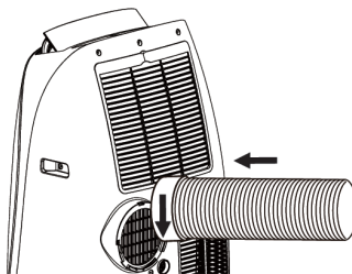
Plastic Hose: Dia. 5.9" (15cm) Length: 14.2" to 47.2" (36cm to 120cm)
