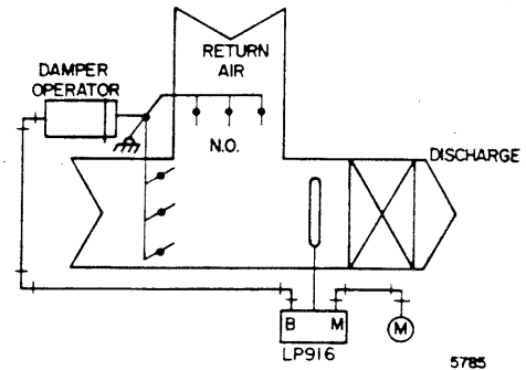
Fig. 3. Typical Mixed Air Application.
