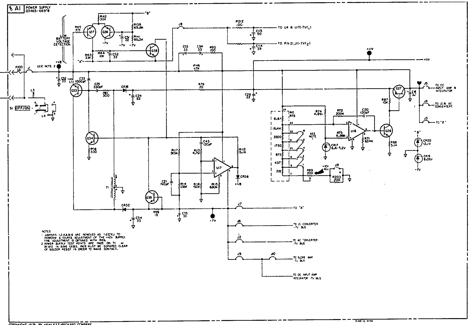
4 Figure 7-5. Power Supply. 7-177-18
