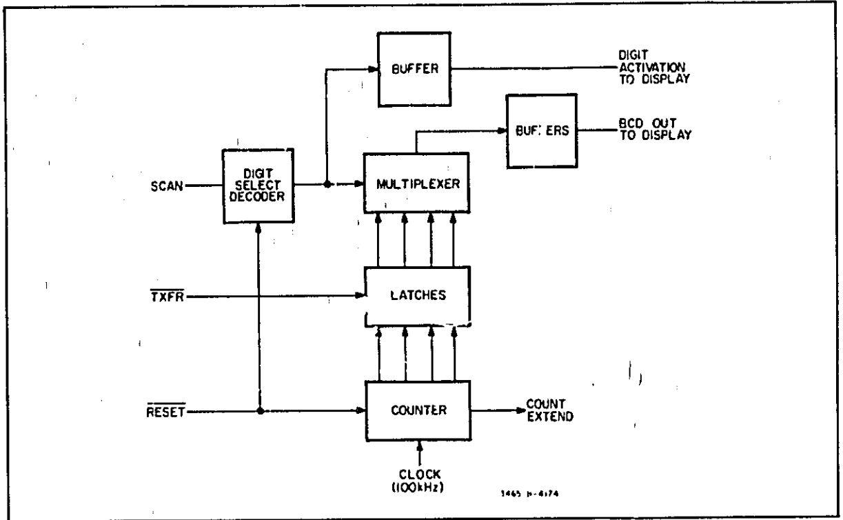
Figure 4-8. Data Accumulator.
