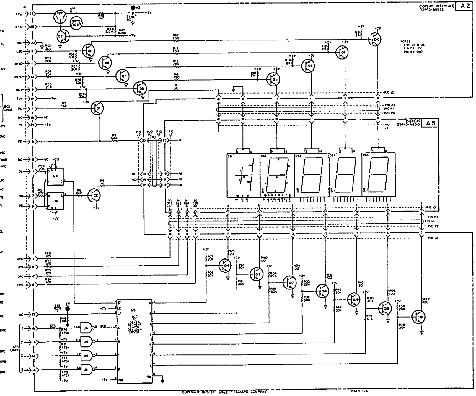
3 Figure 7-4. Logic and Display. 7-15
