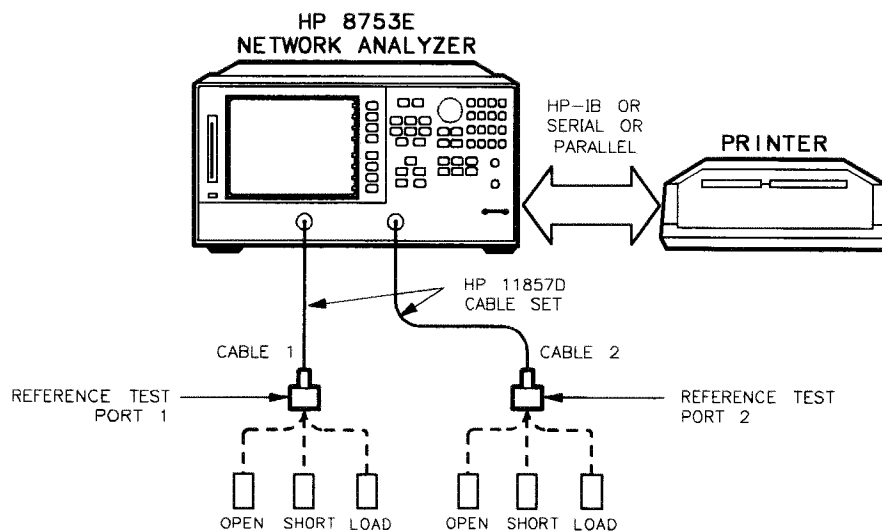
Figure 1-2. Connections for Measurement Calibration Standards
