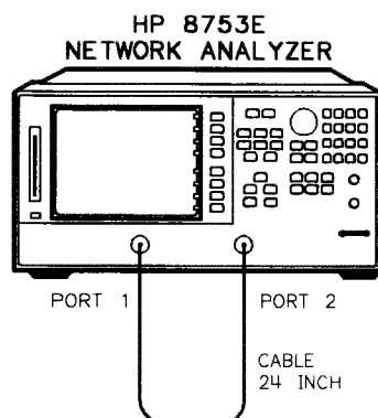
Figure 1-41. Test Port Phase Compression Test Setup
