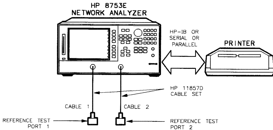
Figure 1-1. System Verification Test Setup
