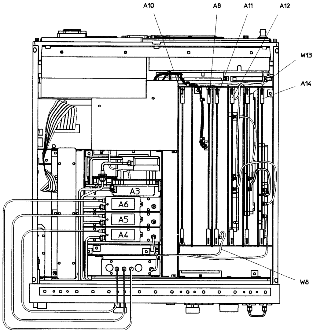
Figure 1-13. Flexible RF Cable Location
