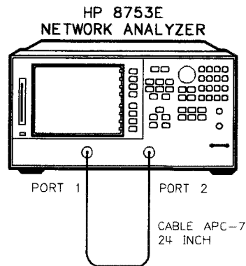
Figure 1-45. Receiver Harmonics Test Setup
