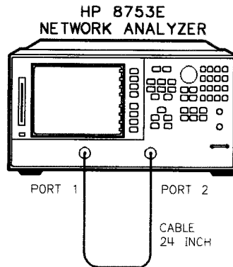
Figure 1-22. Setup for Test Port 1 Input Frequency Response
