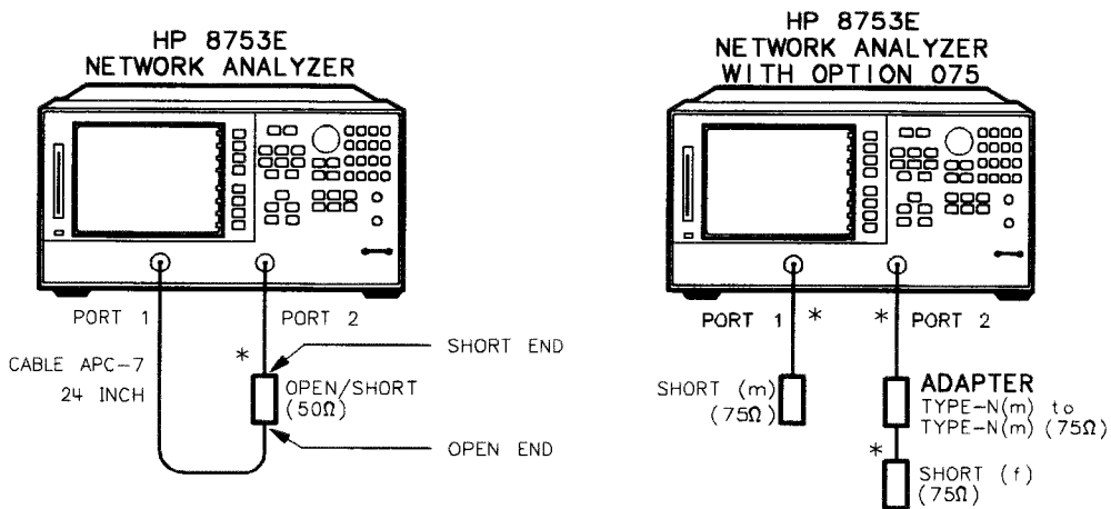
Figure 1-25. Test Port Crosstalk Test Setup
