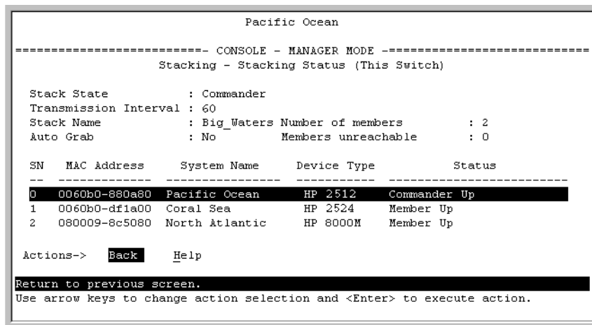
Figure 9-19. Example of the Commander's Stacking Status Screen
