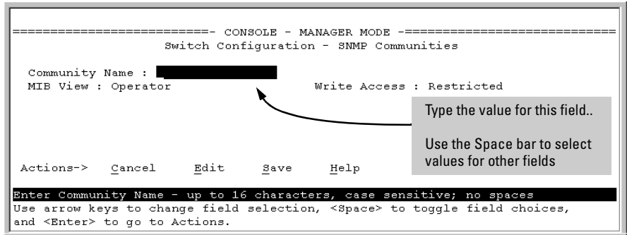
Figure 8-2. The SNMP Add or Edit Screen
