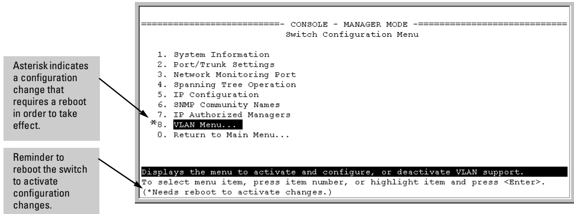
Figure 4-4. Indication of a Configuration Change Requiring a Reboot
