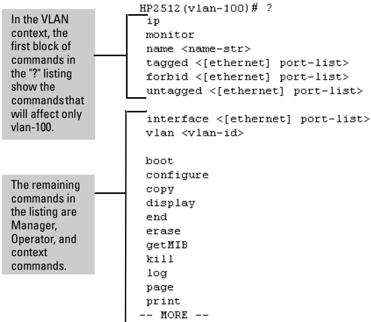
Figure 3-11. Context-Specific Commands Affecting VLAN Context
