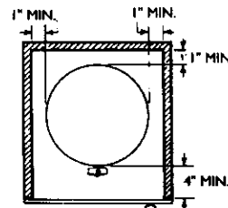
INSTALLATION CLEARANCES TOP VIEW
