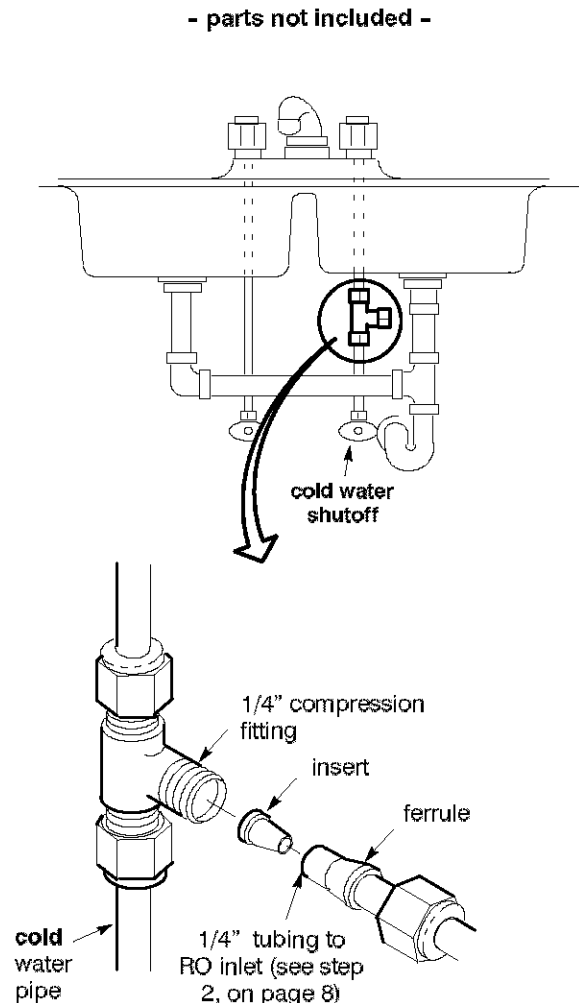
B. WATER SUPPLY TYPICAL CONNECTION (using compression fitting)
