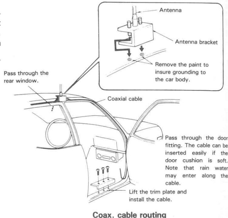
Coax. cable routing
