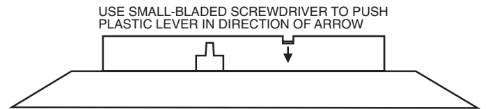
FIGURE 3B. REMOVING DETECTOR HEAD FROM BASE:
