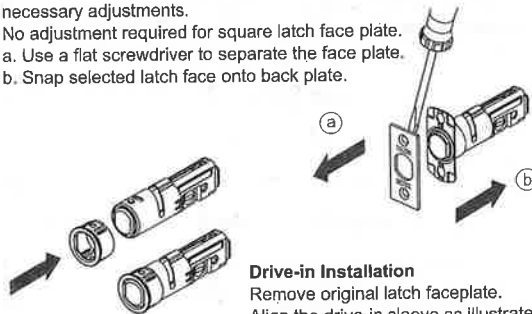
Drive-In Latch
