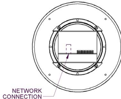
Figure 1. VIP-160A Connections
