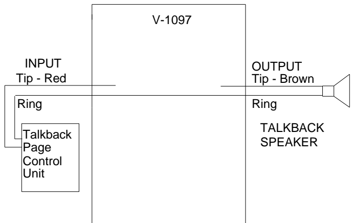
Figure 2. Talkback Connection
