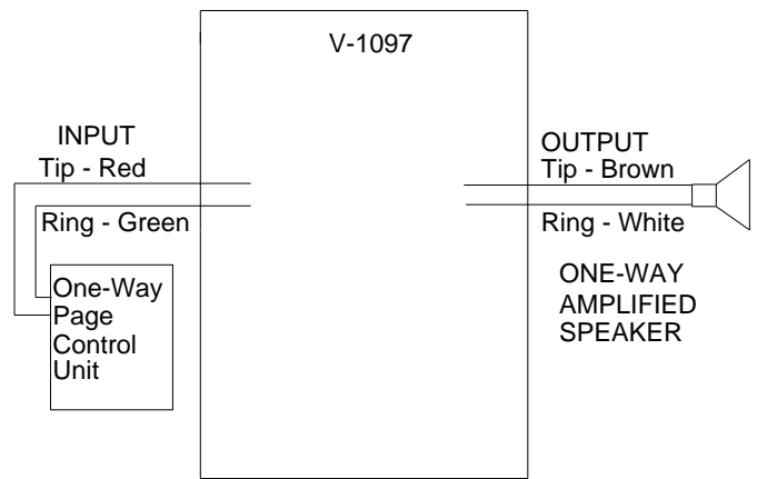
Figure 1. One-Way Connection
