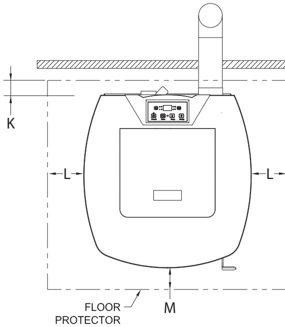
THROUGH THE WALL INSTALLATION
