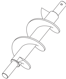
892187 1 Auger
