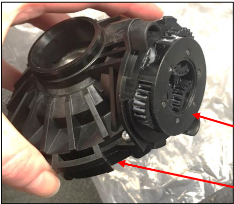
New planet carrier
