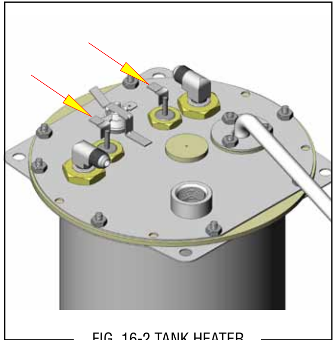
FIG. 16-2 TANK HEATER
