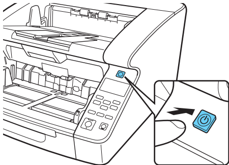
Power Switch
