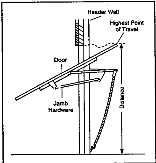
One-piece door without jamb hardware
