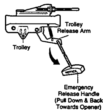
Lockout position
