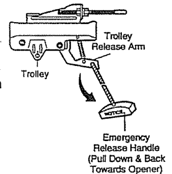
Lockout position
