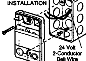
Figure 2 PRE-WIRED INSTALLATION
