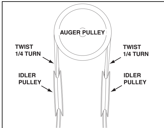
FIGURE 22 VIEWED FROM REAR
