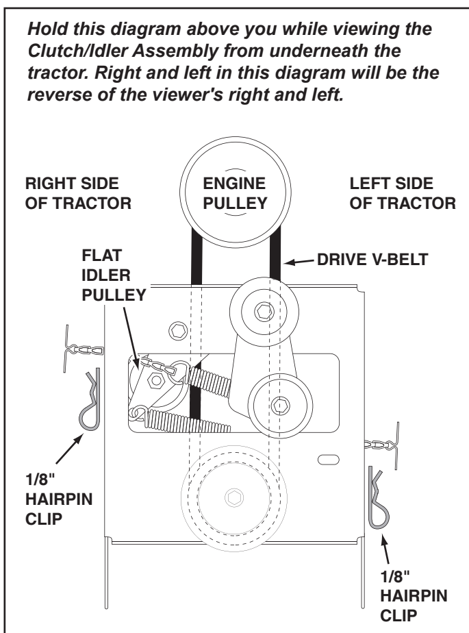
FIGURE 21 VIEWED FROM UNDERNEATH
