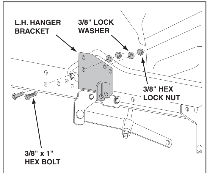
FIGURE 5 LEFT SIDE VIEW
