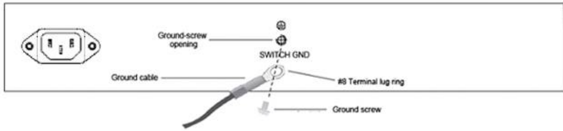
Figure 3-5 – Ground cable, screw and #8 terminal lug rings
