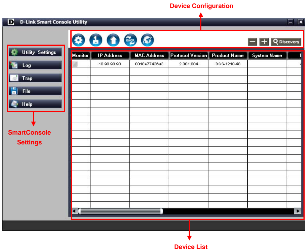
Figure 16 – SmartConsole Utility
