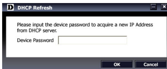
Figure 25 – DHCP Refresh
