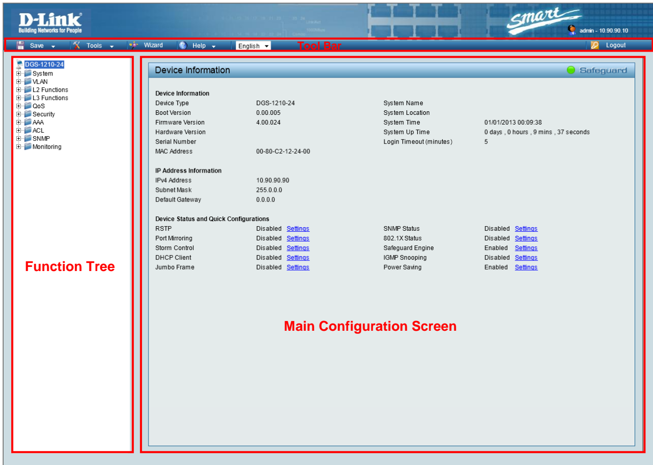
Figure 4.5 – Web-based Management
