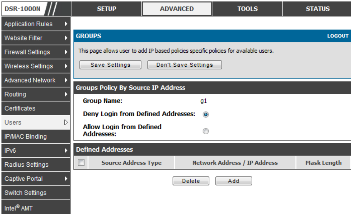
Figure 70: IP policies options
