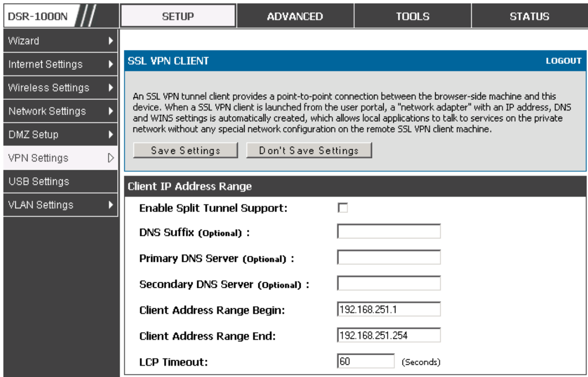
Figure 77: SSL VPN client adapter and access configuration
