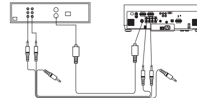
connect S-video and video cables
