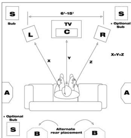
MULTICHANNEL PLACEMENT
