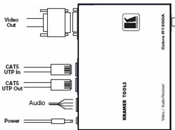
Figure 2: Cobra R1300A Video / Audio Receiver Connections
