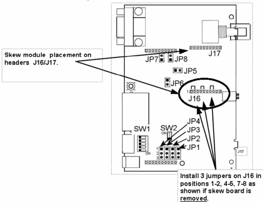
Figure 6: Skew Module
