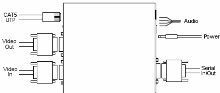
Figure 3: Transmitter Connections
