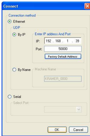
Figure 12: Connect Window
