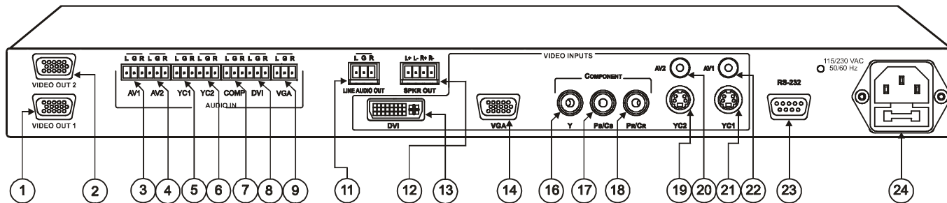
Figure 4: VP-720xl Presentation Switcher / Scaler Rear Panel 2
