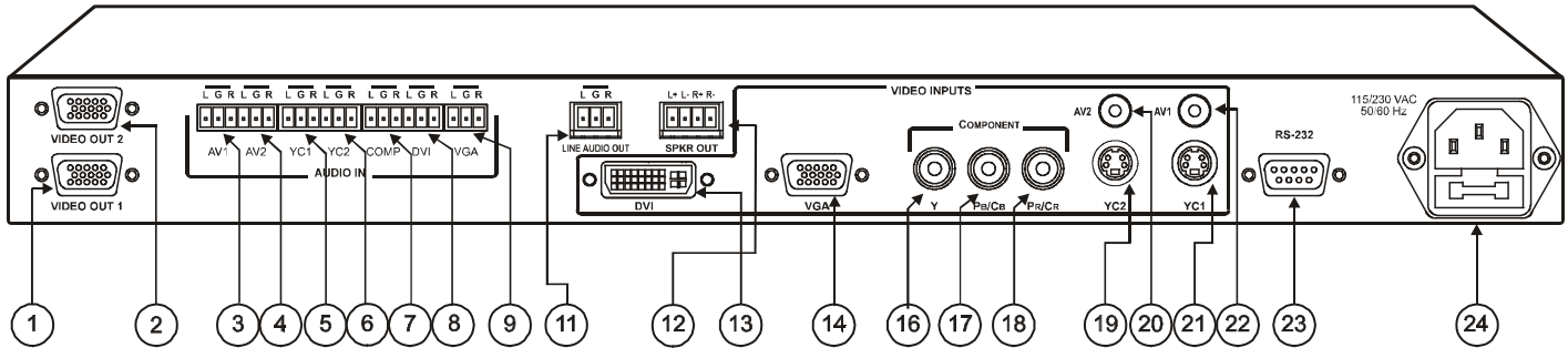
Figure 6: VP-723xl Presentation Switcher / Scaler Rear Panel 2
