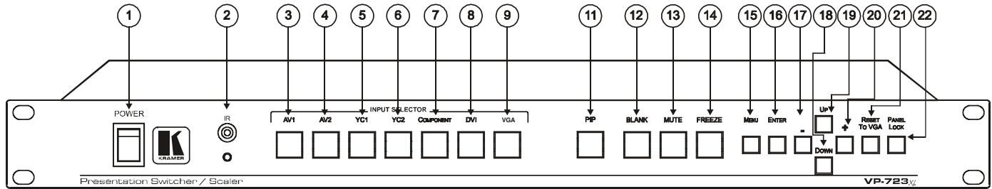
Figure 5: VP-723xl Presentation Switcher / Scaler Front Panel 1
