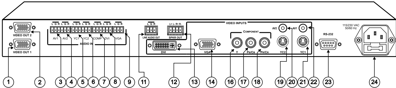
Figure 2: VP-719xl Presentation Switcher / Scaler Rear Panel 2
