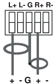
Figure 4: Connecting the Balanced Stereo Audio Output to an Unbalanced Acceptor
