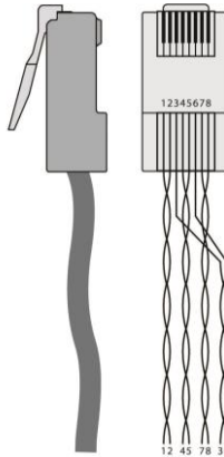
Figure 4: CAT 5 PINOUT
