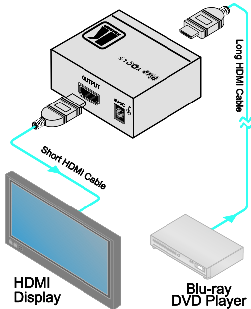
Figure 2: Connecting the PT-101Hxl HDMI Repeater
