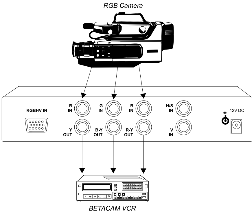
Figure 2: Converting from an RGB Camera to a BETACAM VCR
