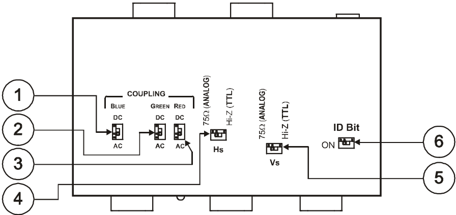
Figure 3: VP-350 1:3 High Resolution UXGA DA Underside
