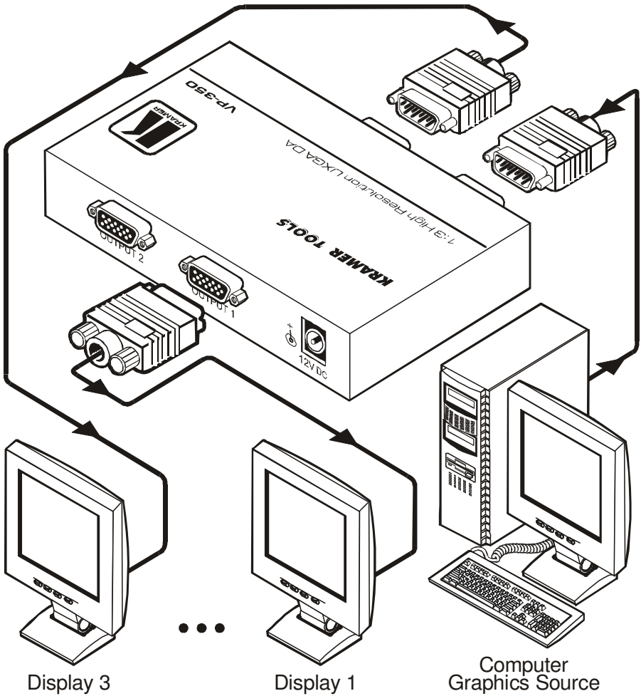
Figure 4: Connecting the VP-350
