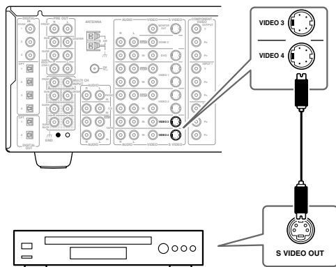
Satellite, cable, set-top box, LD player, etc.
