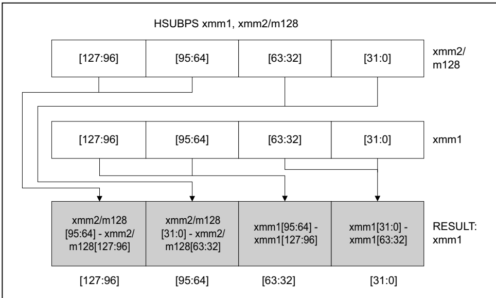
Figure 3-13. HSUBPS—Packed Single-FP Horizontal Subtract
