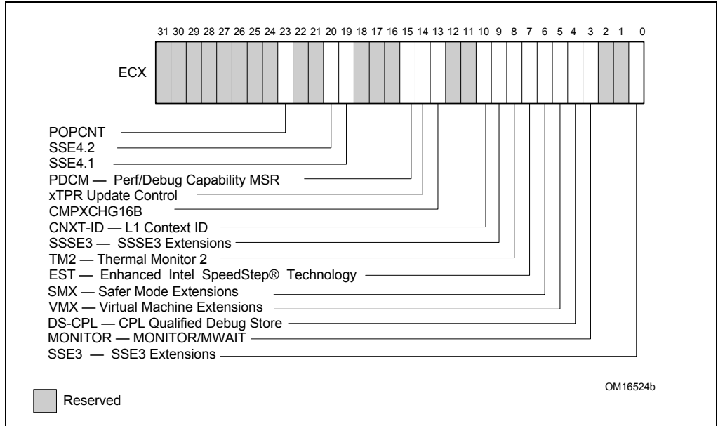
Figure 3-6. Feature Information Returned in the ECX Register
