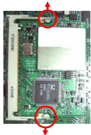
3. to remove the card, please pull out the locker on the socket.
