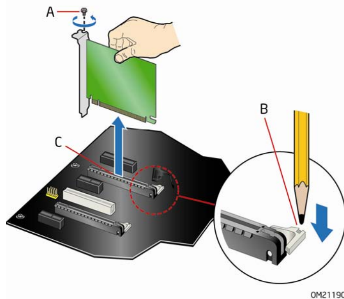
Figure 25. Removing a PCI Express x16 Card
