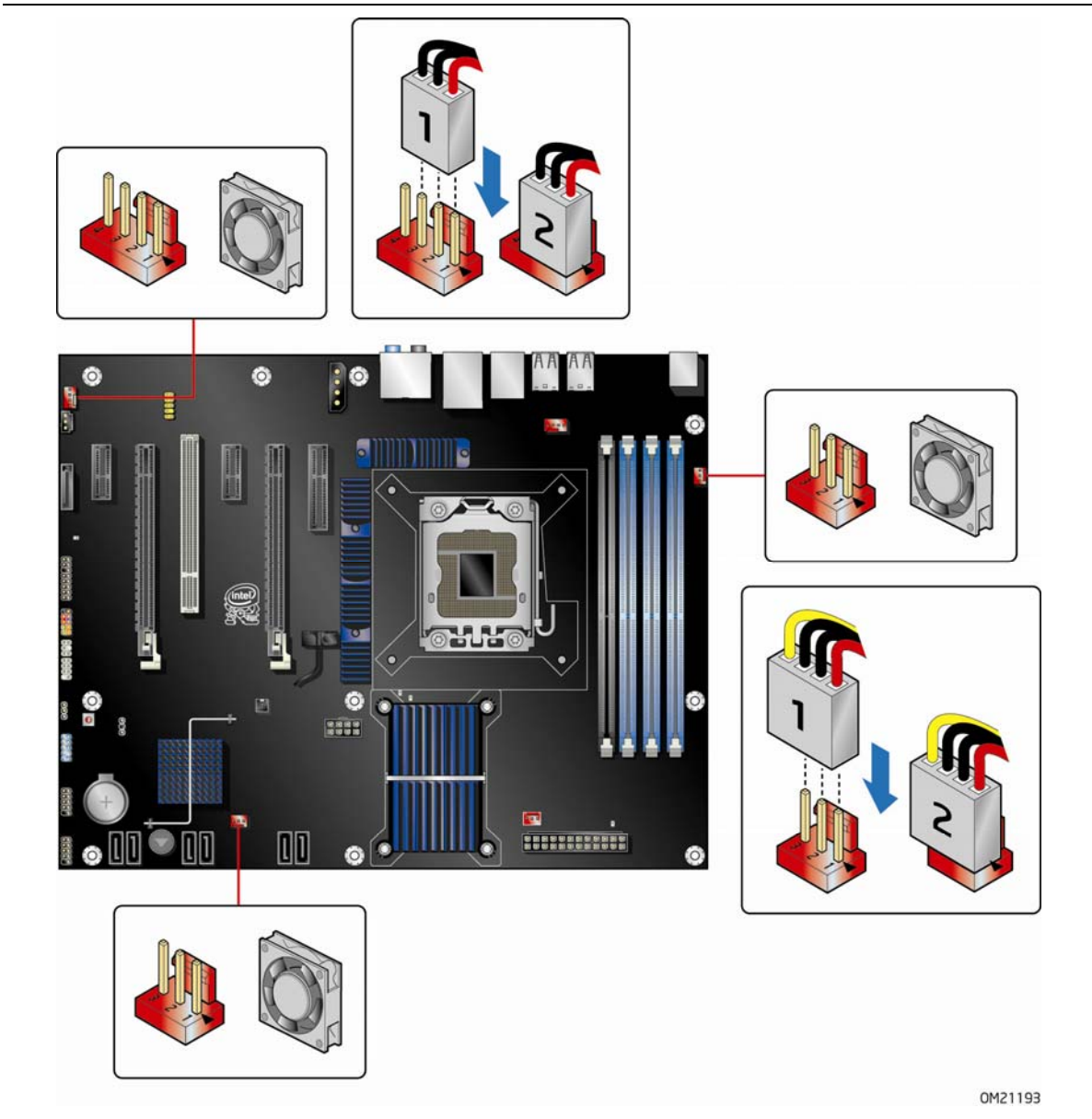
Figure 29. Location of the Chassis Fan Headers
