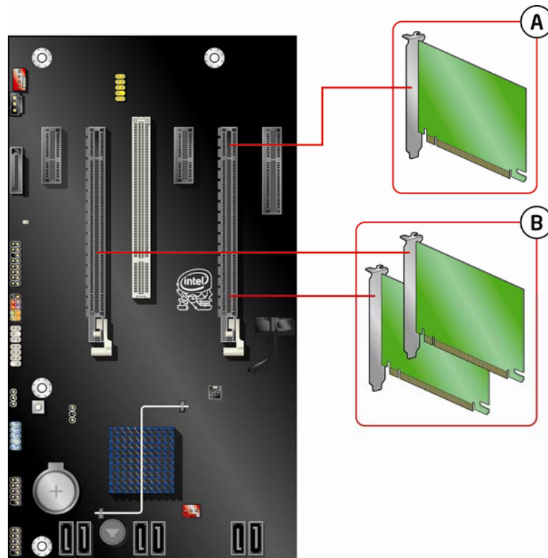
Figure 23. Installing Multiple PCI Express x16 Graphics Cards
