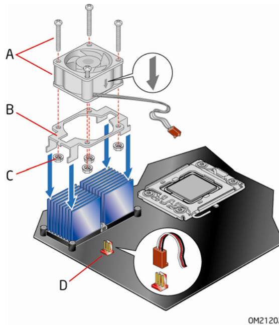
Figure 17. Installing the IOH Fan
