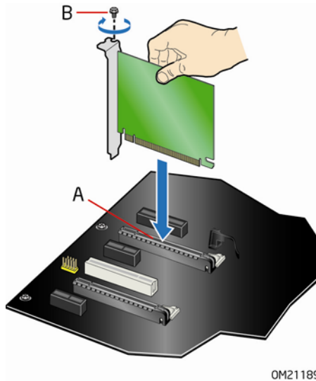
Figure 24. Installing a PCI Express x16 Card
