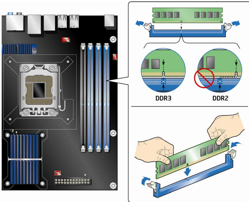
Figure 22. Installing a DIMM
