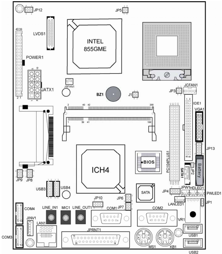
PPC-7508F Connector, Jumper and Component locations
