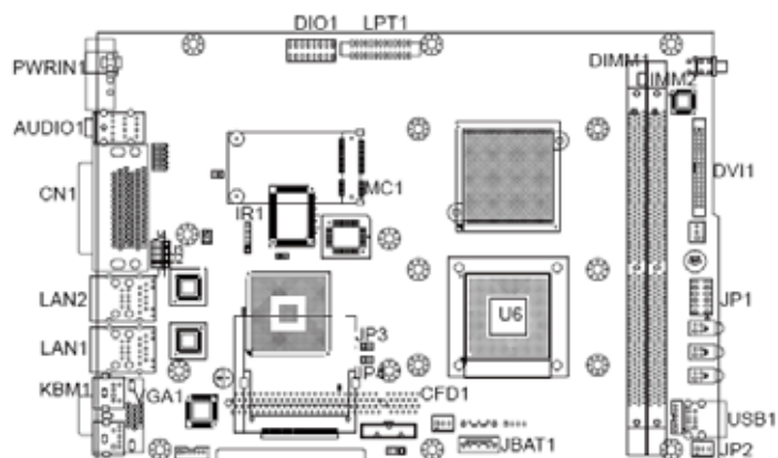
Figure 2.1: EX-98211 Main Board Top View
