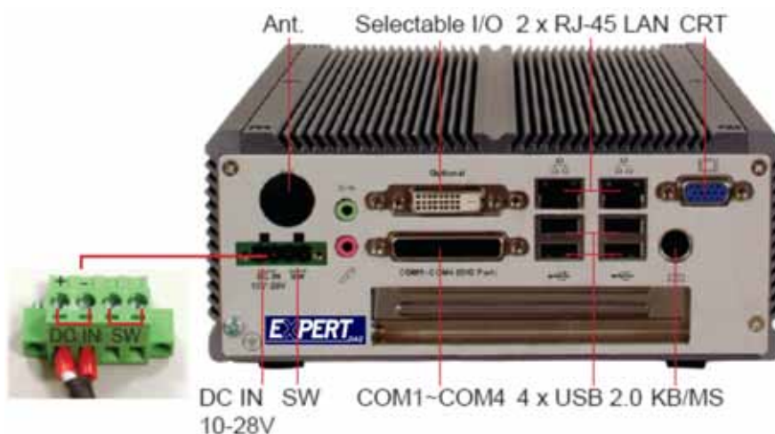
Figure 1.2: Back View of EX-98211
