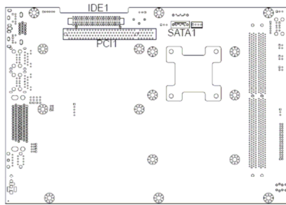
Figure 2.2: EX-98211 Main Board Bottom View
