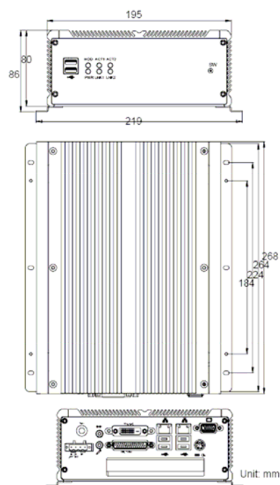
Figure 1.3: Dimensions
