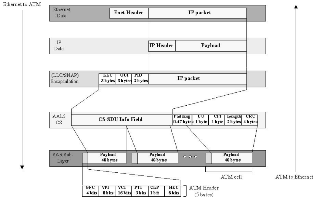
Figure 1 – Protocol Processing
