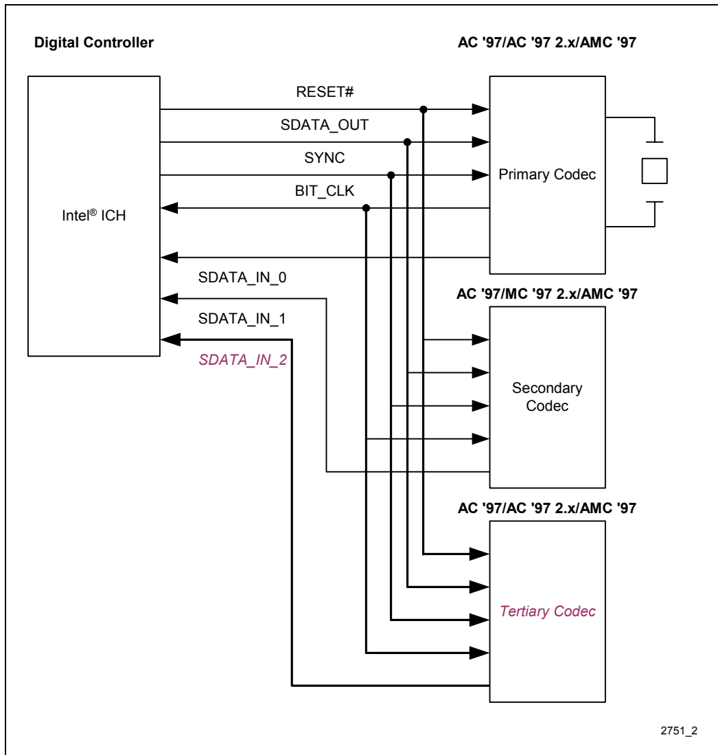
Figure 2. Intel® ICH5 AC '97 Controller Connection to Its Companion Codecs
