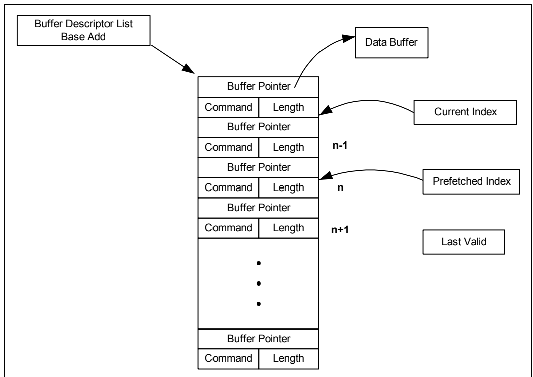
Figure 4. Buffer Descriptor List
