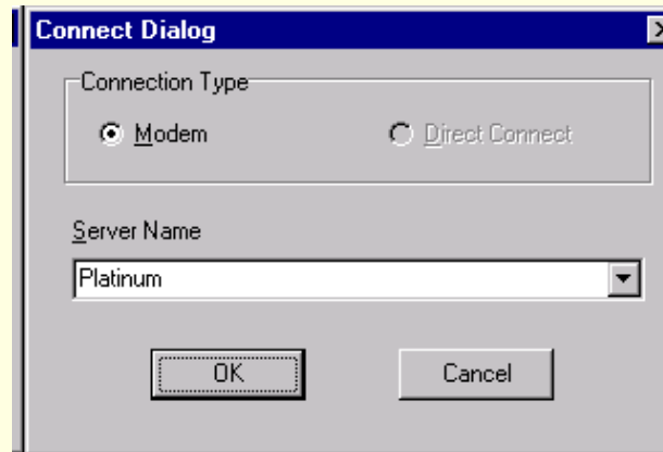
Connect Dialog
