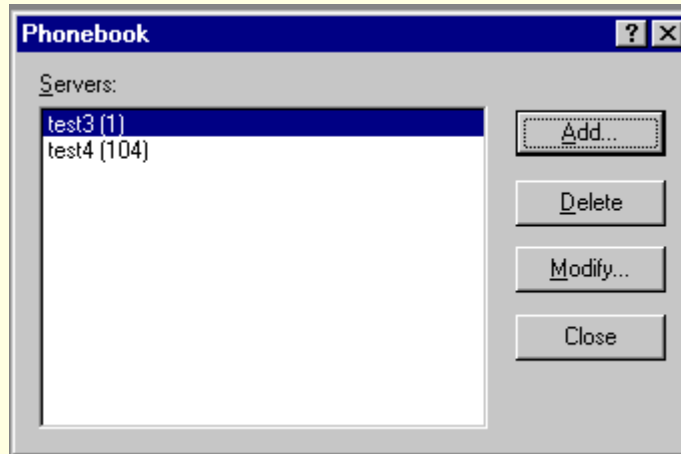
Phonebook Dialog
