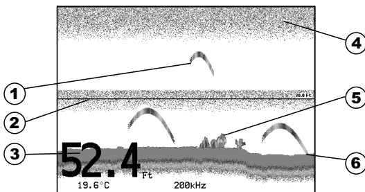
Fig. 2.1.1 - The Fish Finder Display
