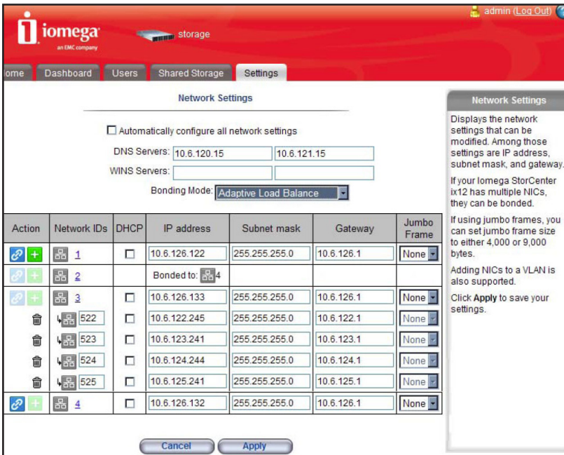
Figure 5 Bonded network interface
