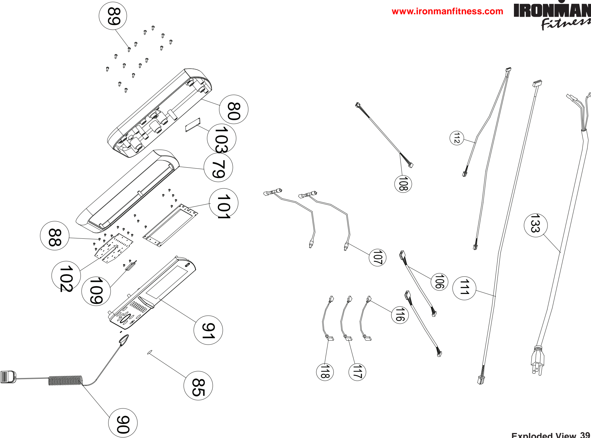
Exploded View 39
